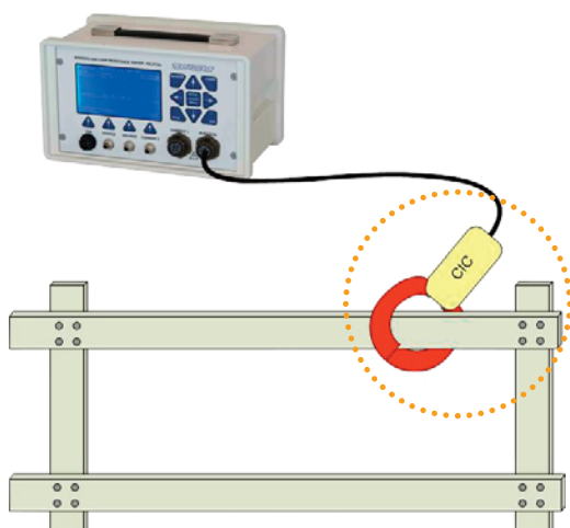
Loop Resistance Test (Option L, M, N) Single Clamp Measurement
